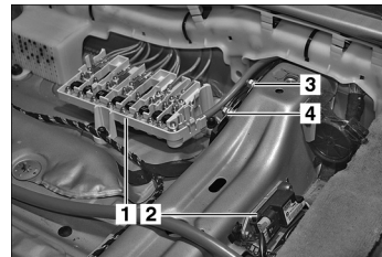
Locations of hundreds of electrical components: Fuse panel under passenger seat. ECL Electrical Component Locations
